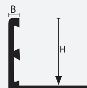
TR 175-225 0* B = 3 mm
